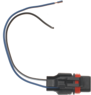
65-168P Back-Up Lamp Connector 19368709; 1U2Z14S411YA; F4SZ14489A; 12102664
